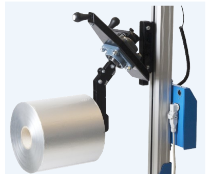
Manual expander for lifting and rotating small rolls within the core.
